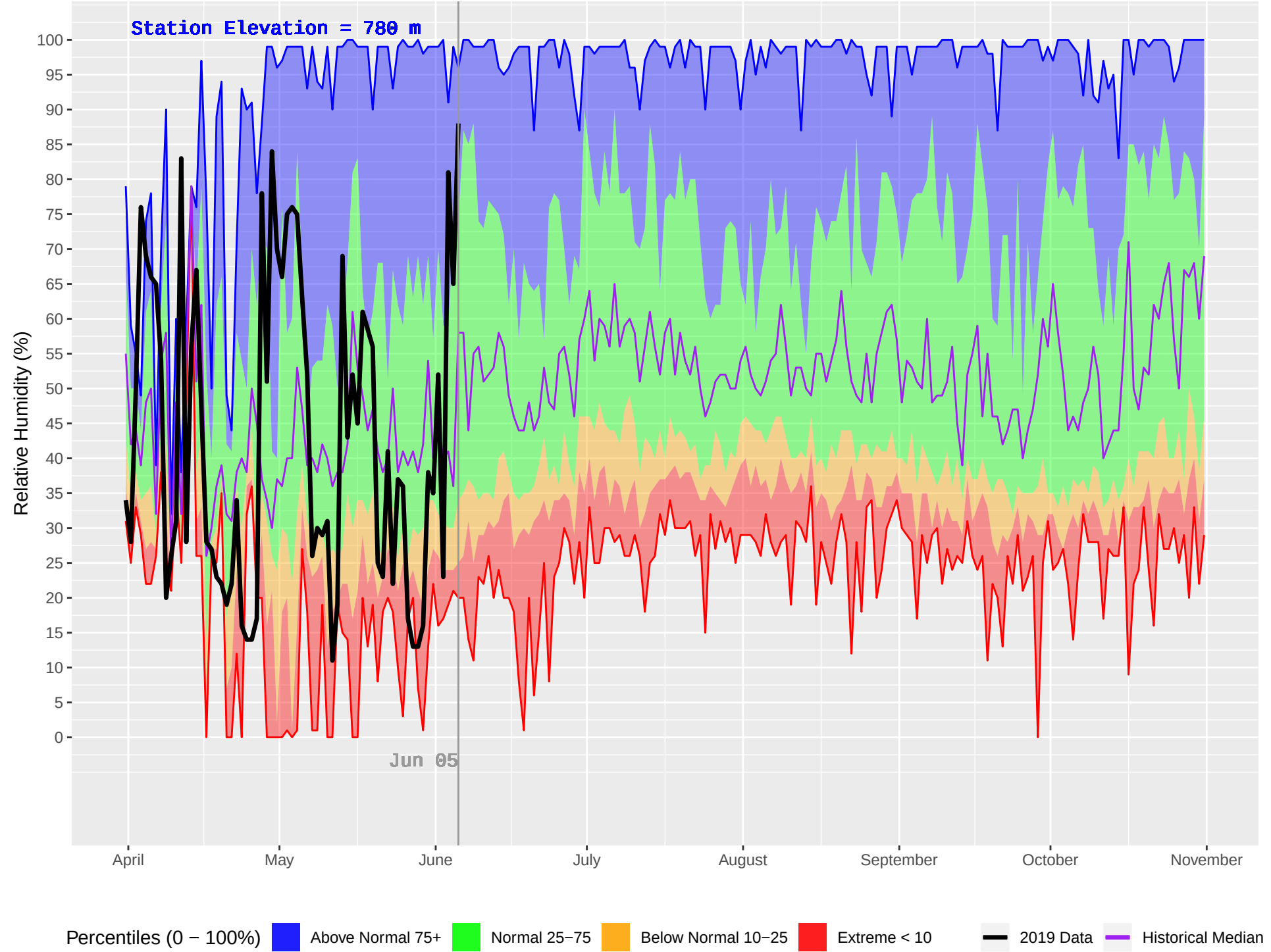
MUSKWA (131) : Historical (1983–2018) and Current (2019) Daily Relative Humidity
