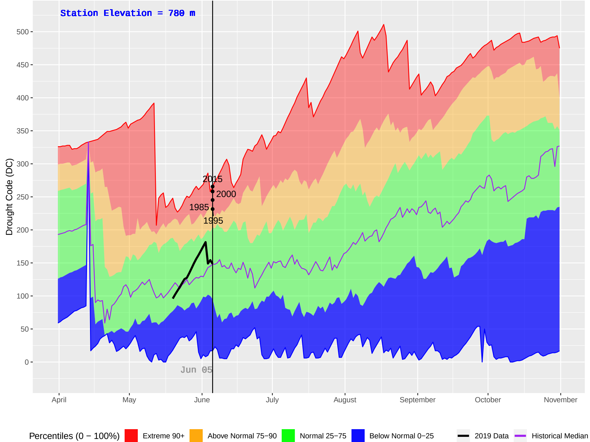
MUSKWA (131) : Historical (1983–2018) and Current (2019) Daily Drought Code (DC)
