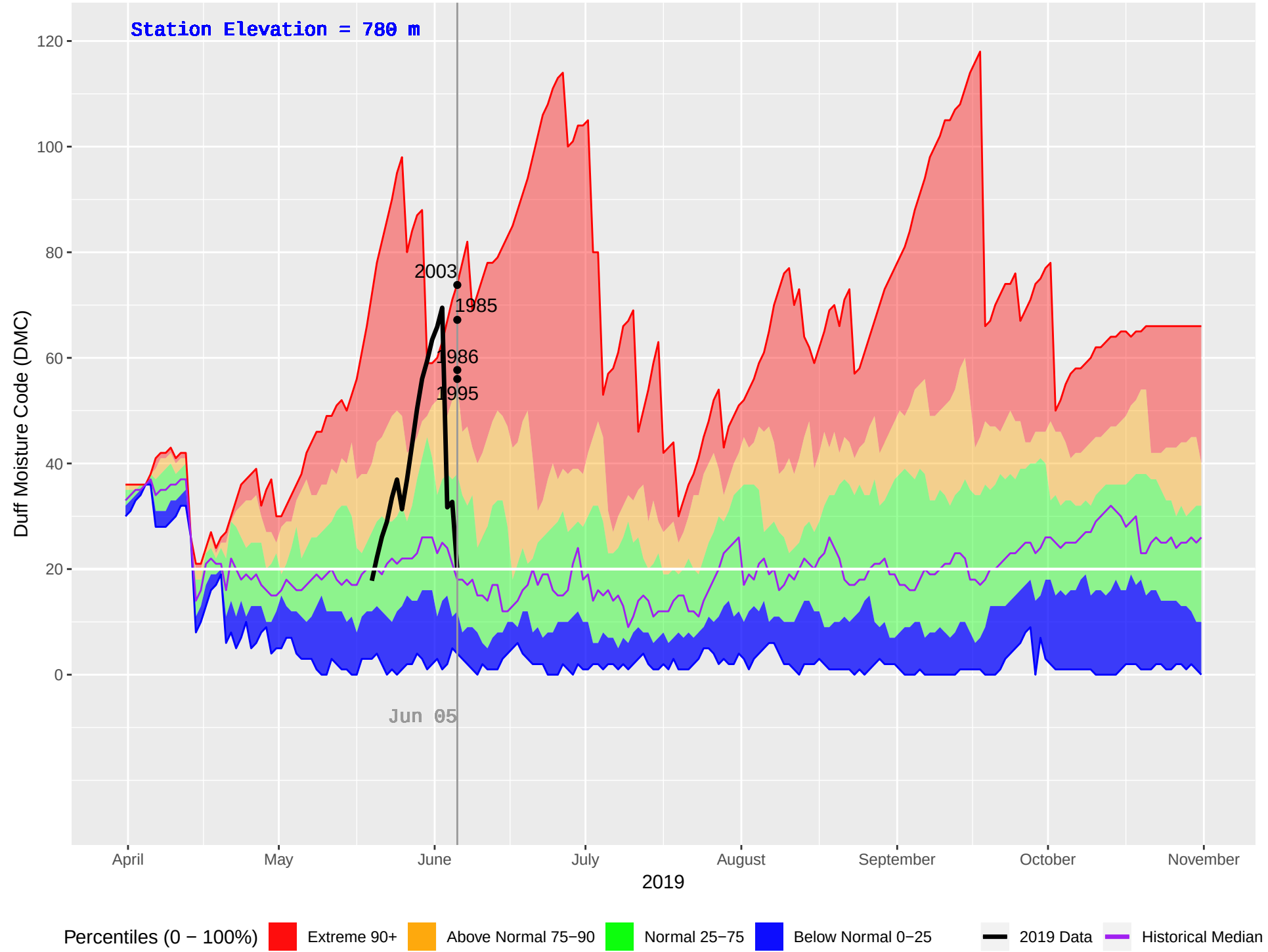
MUSKWA (131) : Historical (1983–2018), Current (2019) Daily Duff Moisture Code (DMC)
