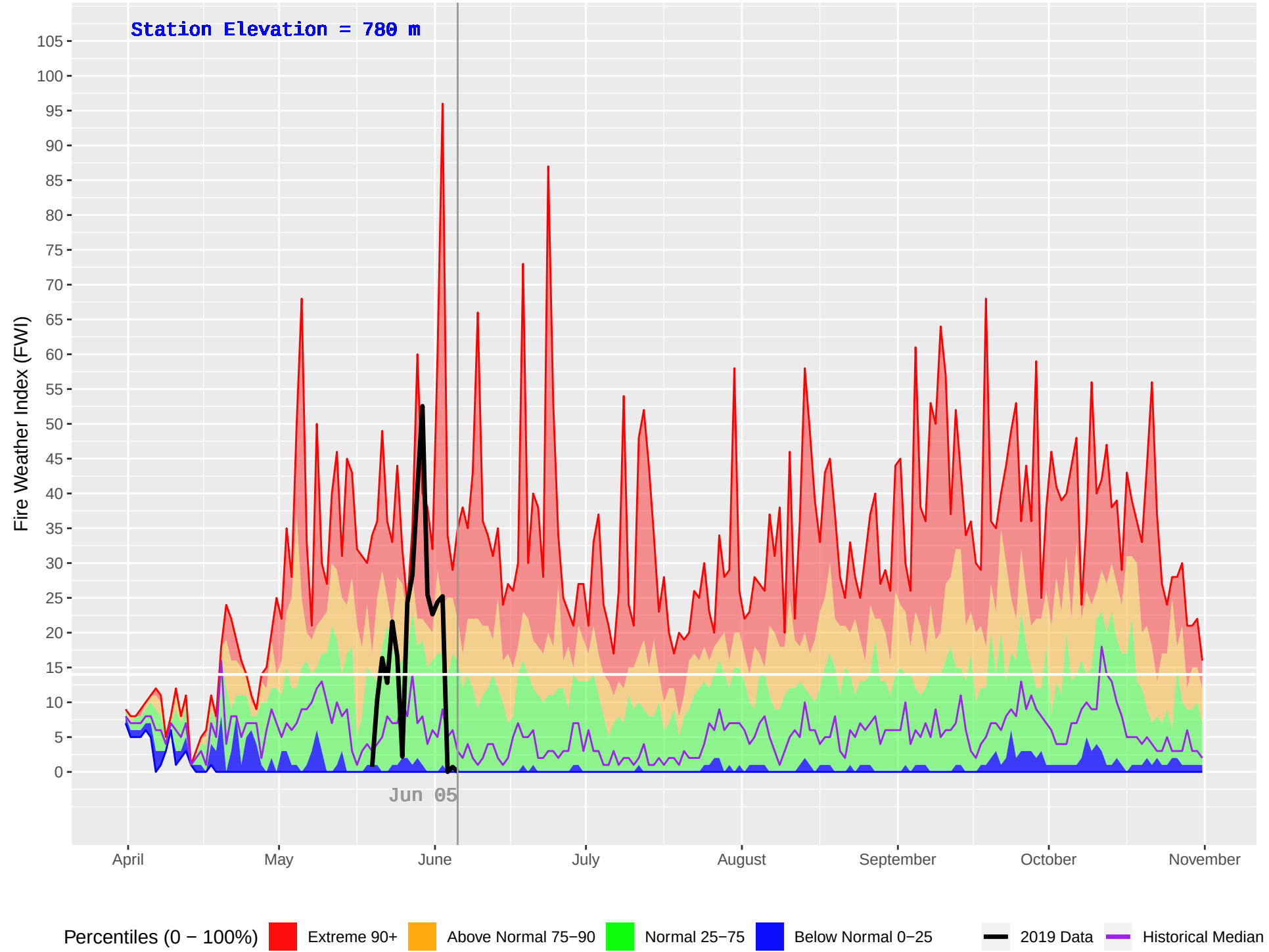
MUSKWA (131) : Historical (1983–2018) and Current (2019) Daily Fire Weather Index (FWI)
