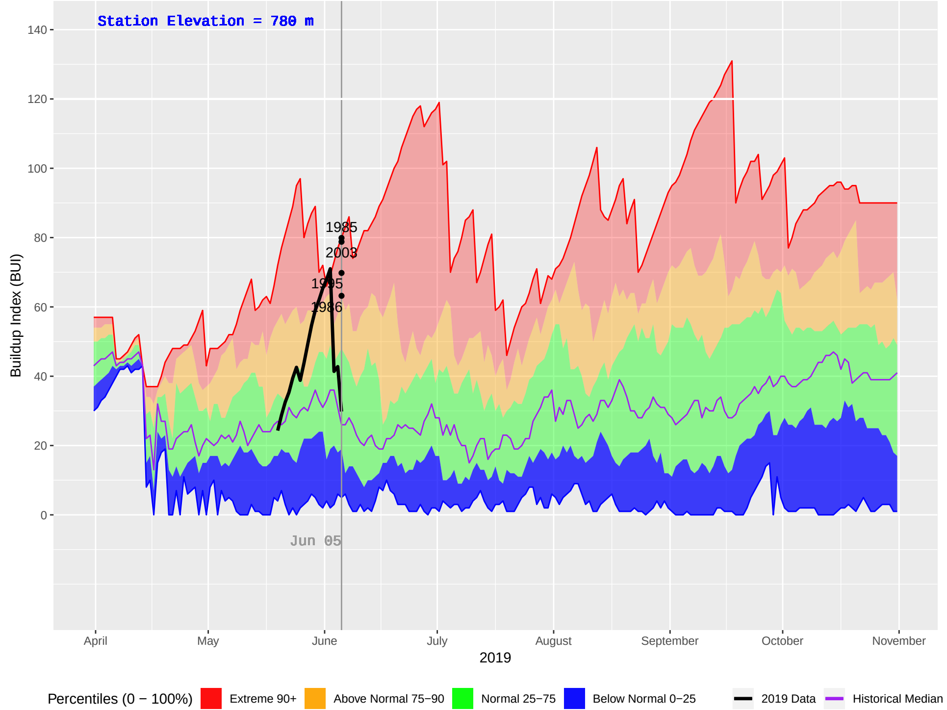
MUSKWA (131) : Historical (1983–2018), Current (2019) Daily Buildup Index (BUI)
