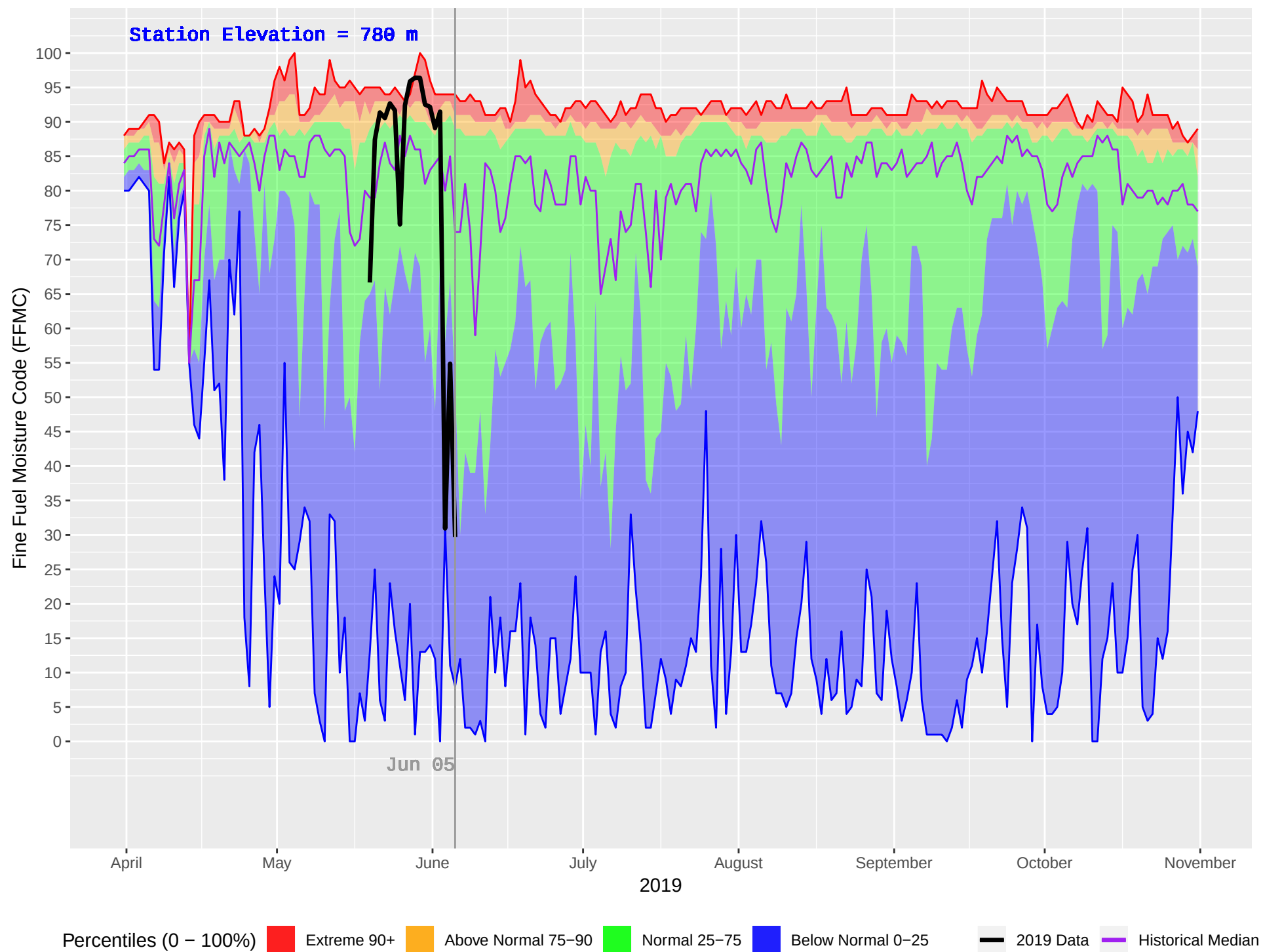
MUSKWA (131) : Historical (1983–2018) and Current (2019) Daily Fine Fuel Moisture Code (FFMC)
